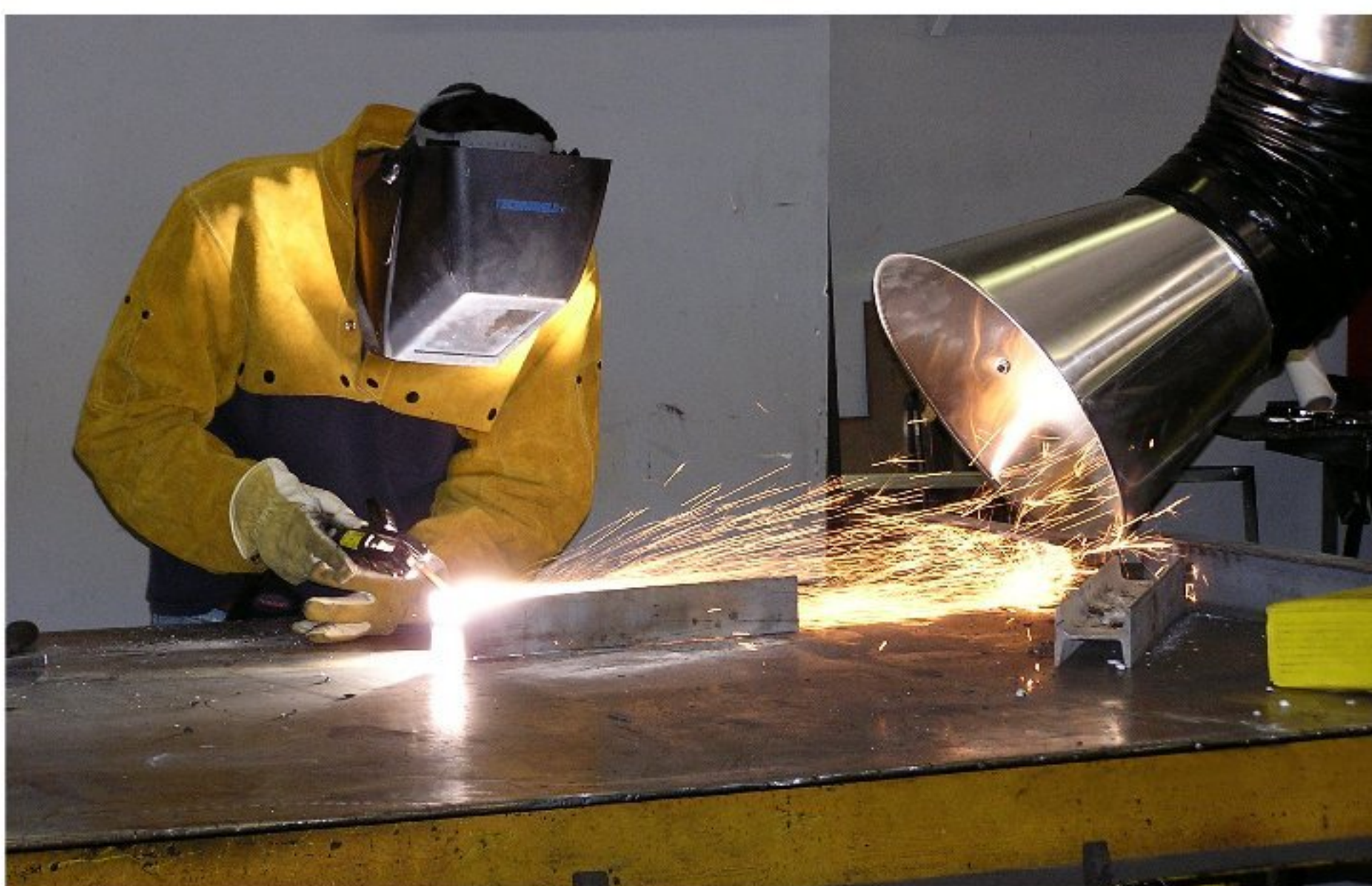
Impinger Spark Trap Prevents Sparks From Entering Collector
